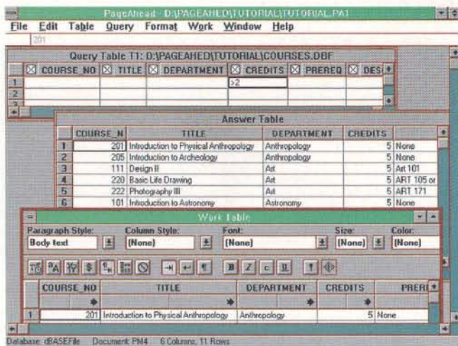
Screen 2: PageAhead uses a spreadsheet-like interface. In the Query Table (top), you select records; the Answer Table (middle) shows you the results; and the Work Table is where you specify text formats and styles.
